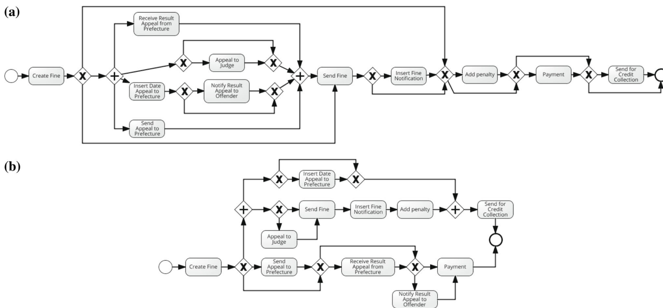
Fig. 18 Comparison of process models that are mined with the default parameters and with the parameters that maximize the geometric average of replay fitness and precision. The process is concerned with road-traffic fine management and models are represented using the BPMN notation. a Model mined using the Inductive Miner with default
