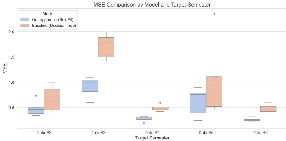
Fig. 7 Comparison of predictive performance between the proposed approach and decision tree baseline, measured in terms of Mean Squared Error (MSE) across 5-fold cross-validation
