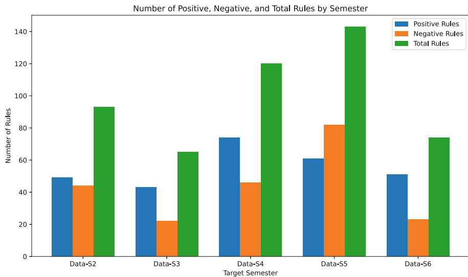
Fig. 8 The number of rules extracted from predictive models for different target semesters
